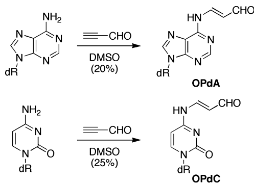
SCHEME 3 One-pot syntheses of OPdA and OPdC.
