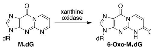
SCHEME 1 Metabolic oxidation of M 1 dG.
